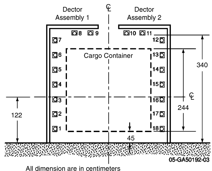
Fig. 3. End view of the cargo container inspection configuration.
