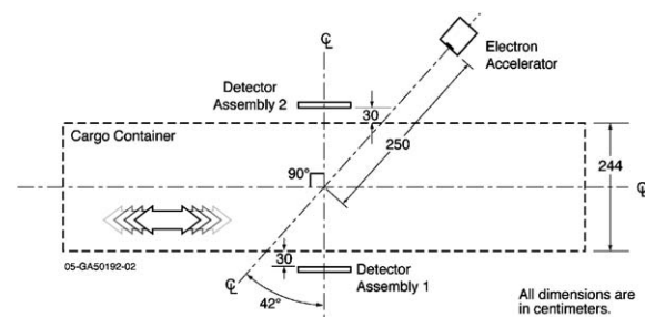
Fig. 2. Top view of the cargo container inspection configuration.
